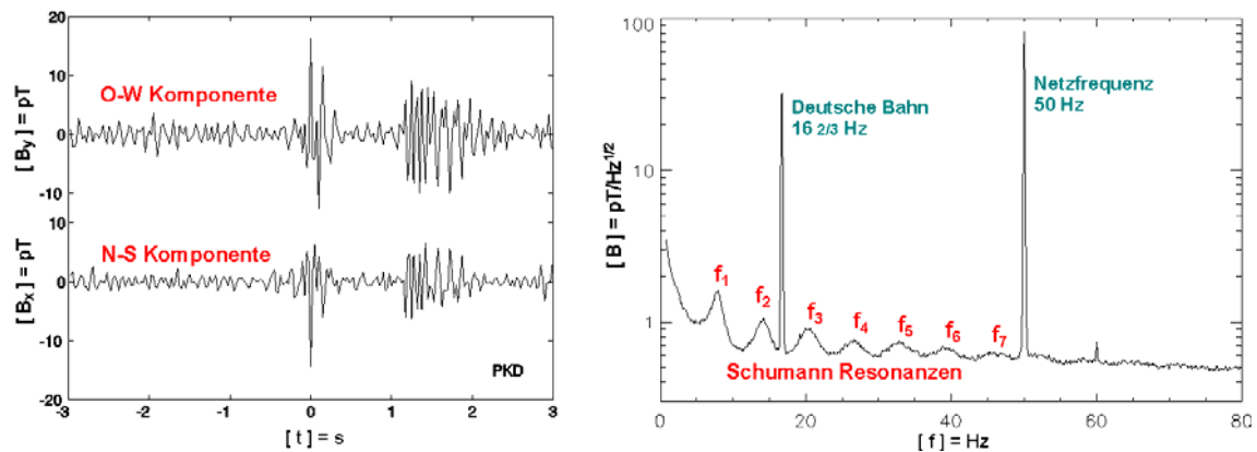
Fig. 2 Time signal (left) and spectrum (right) of the first 7 Schumann resonances measured at Silberborn in Solling Mountains (Germany). Although the nearest electric railway is about 30 km away, the 16 2/3 Hz and the mains frequency signals are much stronger than the Schumann resonance. The increase in the spectrum at frequencies <5 Hz is caused by so-called magnetic micropulsations which originate in the earth's magnetosphere.
