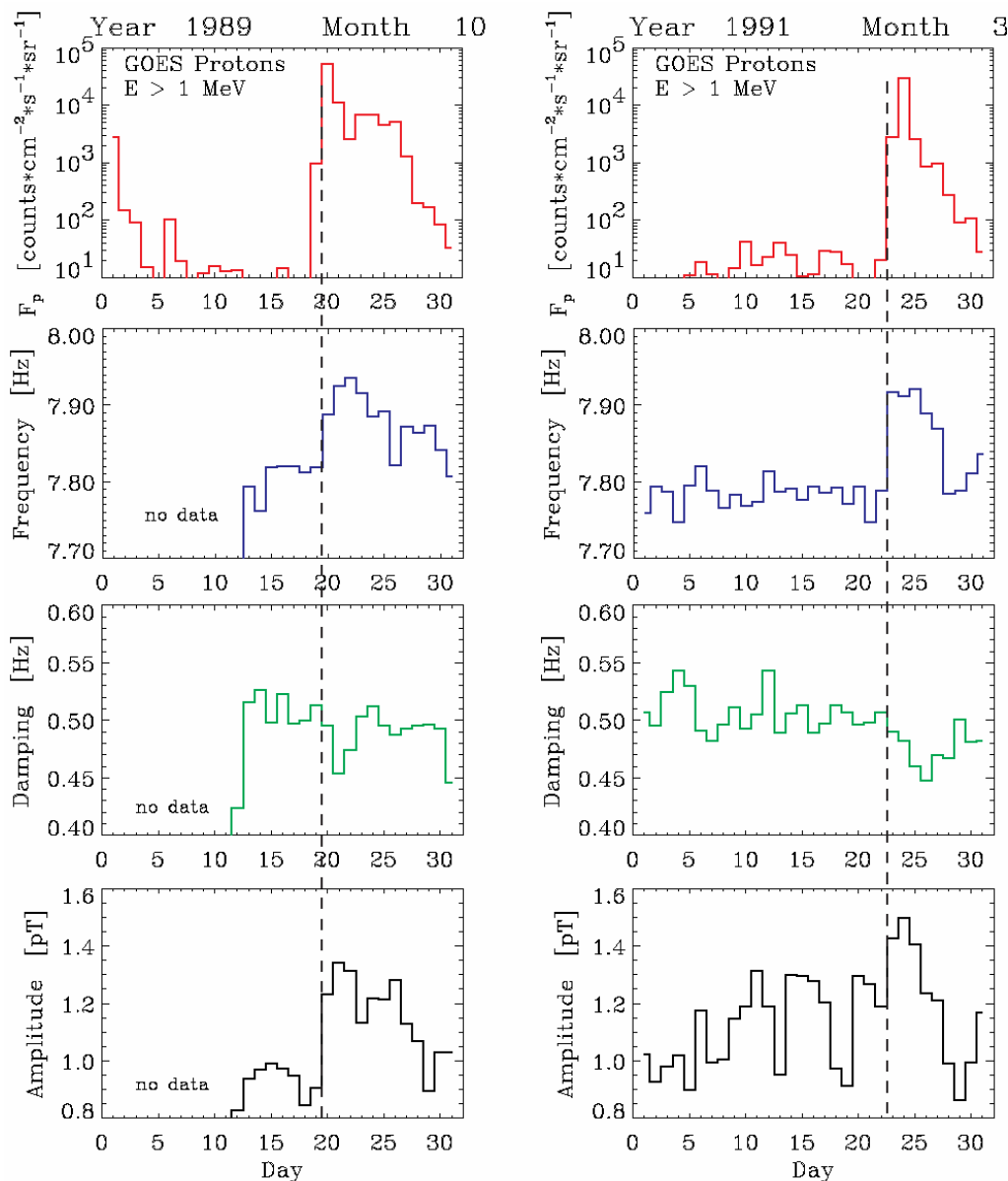
Fig. 9 Changes in Schumann resonance parameters f_0 , b , a (cf. fig. 3) after two solar flares from 20.10.1989 (left) and from 22.3.1991 (right). Directly above the flux of high-energy protons is shown, which cause the additional ionisation below 80 km and thereby change the conductivity as shown in fig. 8 [9].
