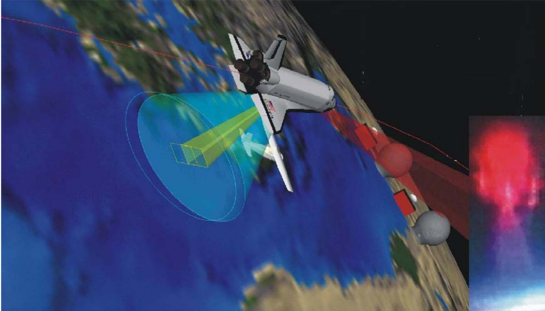
Fig. 7 From the space shuttle an Israeli astronaut will search for sprites and natural gas discharges in the mesosphere with a video camera. On the right below the original photo of a sprite is inserted (the picture was created with STK Software. With approval of M. Moalem, IAF).
