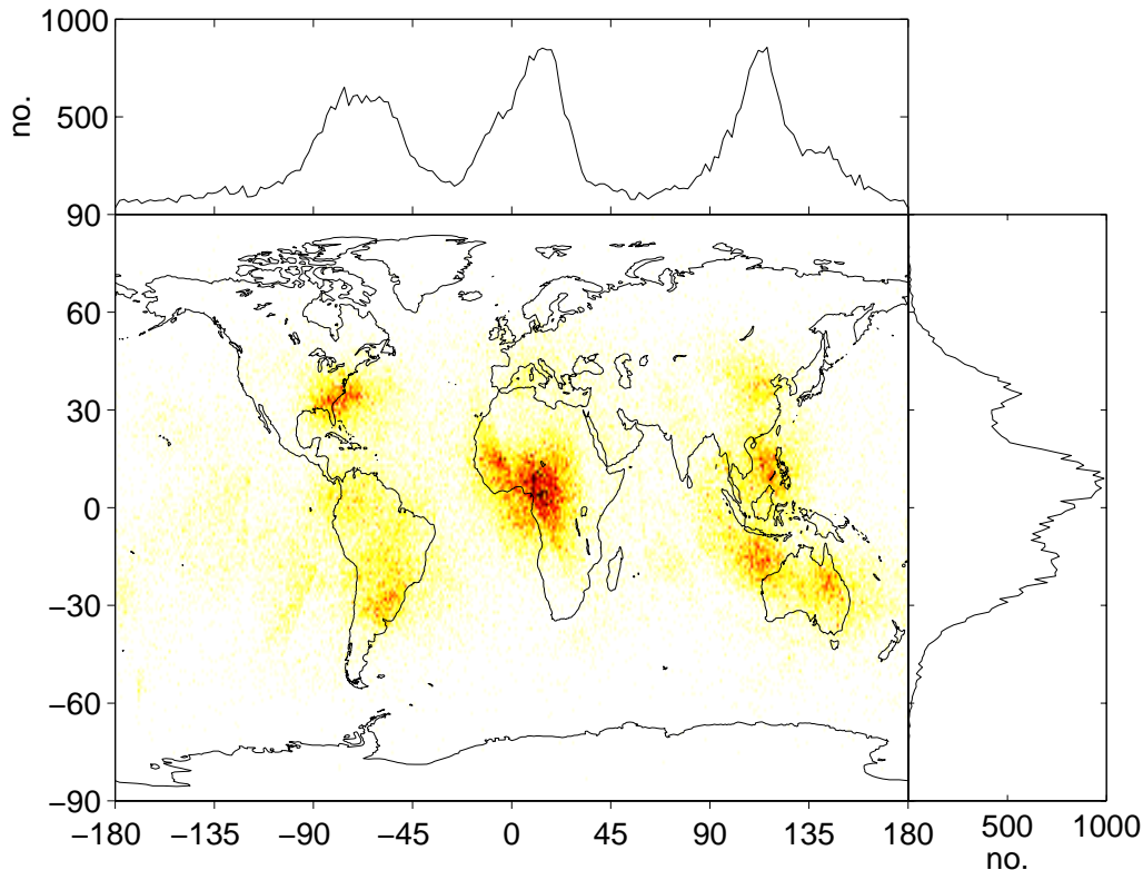
Fig. 6 The global distribution of flash frequency in April 1998 recorded with the help of Schumann resonance triangulation. There are generally three centres with increased flash frequency: over America, Africa and Southeast Asia, while only few thunderstorms appear over the oceans.
